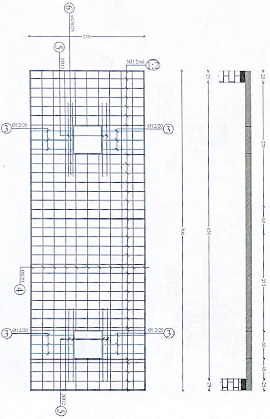
SOLETA B/A(C16/20) SHK.1:50
