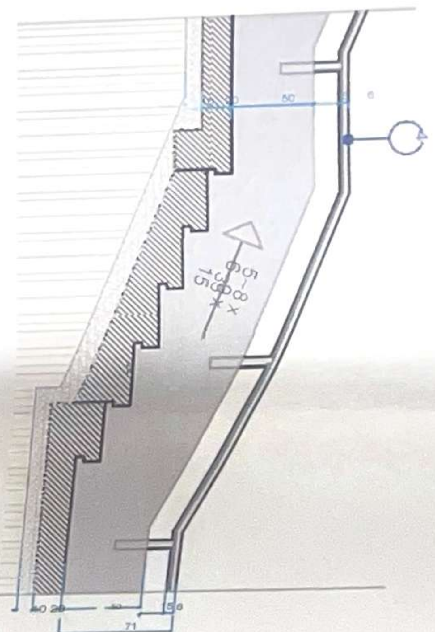
pos 4 shk 1 25
