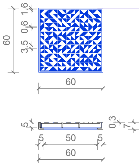
Mbulese gize Model Anti rreshqites /Cast Iron Cover Anti slib pattern 600x600x50
